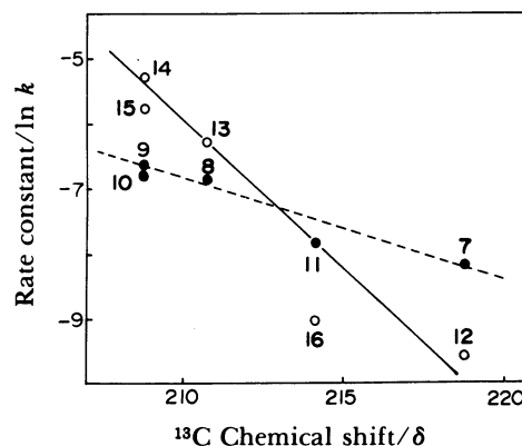
Fig. 3. Correlation of the rate constants of the oxidation of cycloalkanols ( k_{+1} ; \bullet ) and the reduction of cycloalkanones ( k_{-1} ; \circ ) with the ^{13}\text{C} NMR chemical shift of the carbonyl carbon of the cycloalkanones involved in the reaction.
